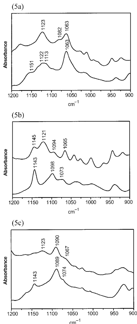
Figure 5. IR spectra (1200–900- \text{cm}^{-1} region) of compounds 9 (5a), 10 (5b) and 12 (5c) in H 2 O (upper spectra) and D 2 O (lower spectra)
